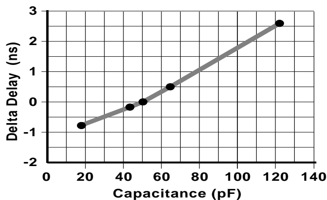
Figure 7: Delay Factor at Various Capacitive Loads X8257
