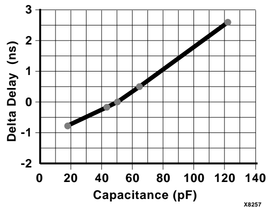
Figure 8: Delay Factor at Various Capacitive Loads
